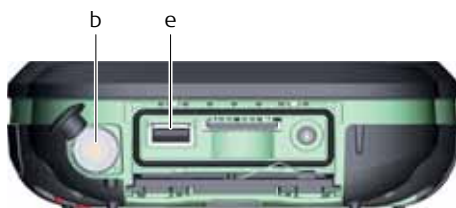
CS20 Controller
