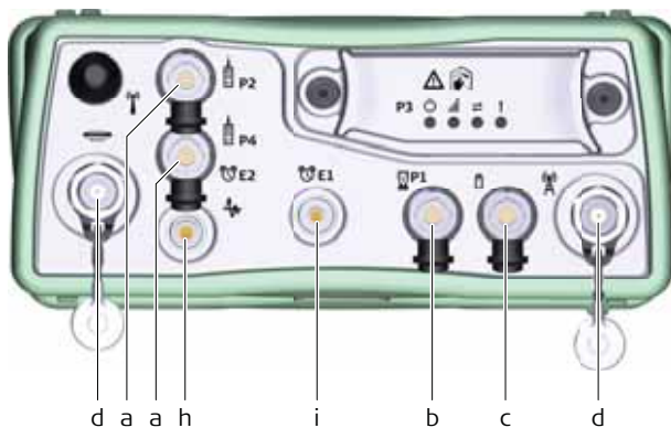
GS16 Receiver
